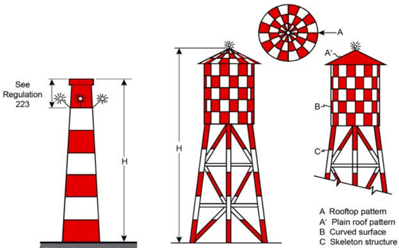
Figure 38: Marking and lighting of tall structures
