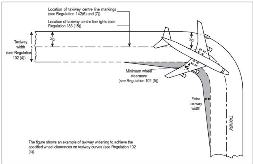
Figure 2. Taxiway curve
