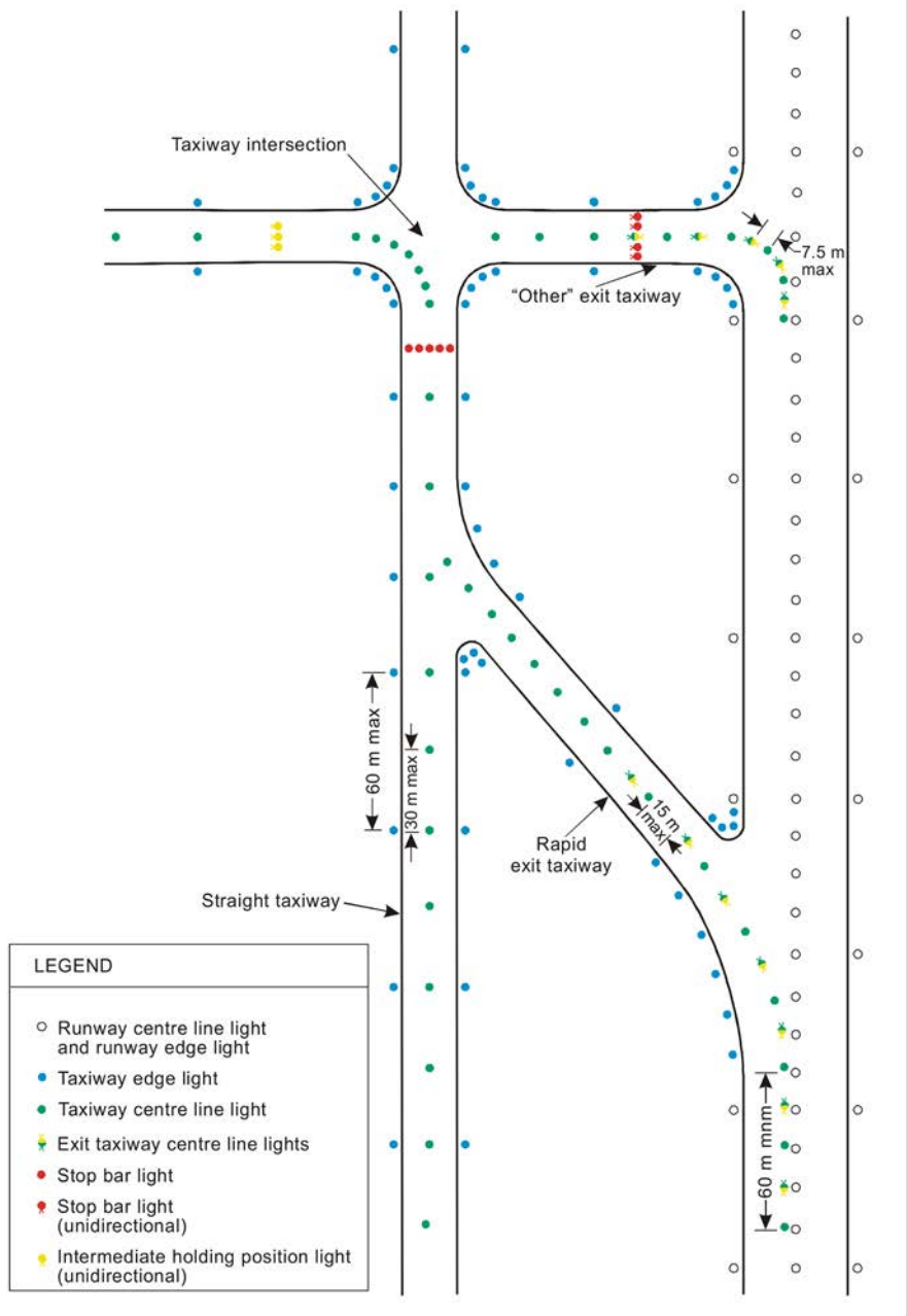
Figure 29: Taxiway lighting
