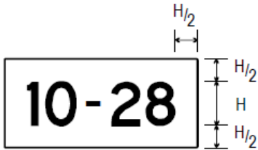
A. Sign with two runway designators
