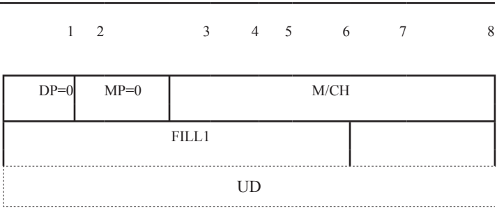
Figure 4-22 Long Form MSP Packet
