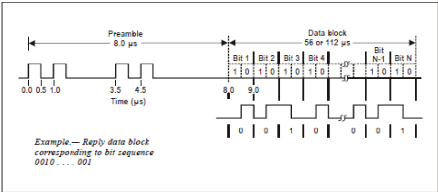
Figure 4-5. Mode S reply
