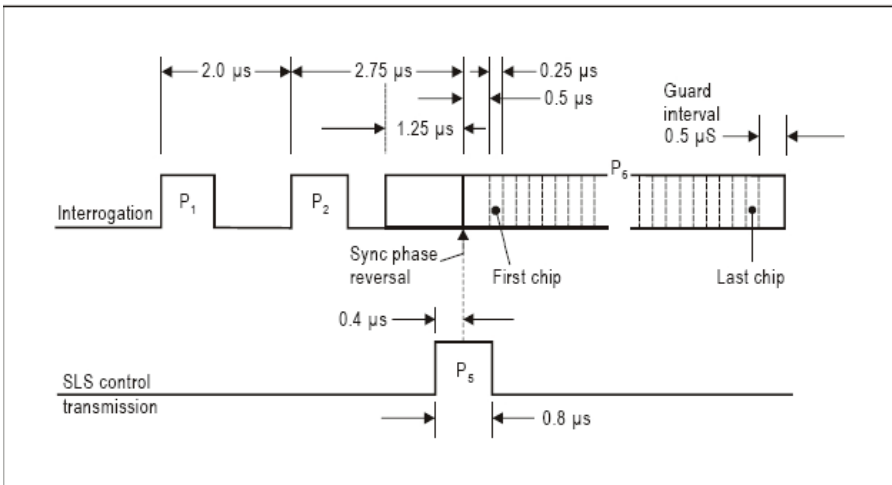
Figure 4-3 Mode S interrogation pulse sequence.
