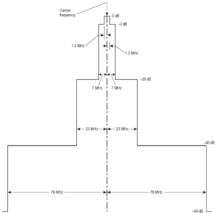
Figure 4-4. Required spectrum limits for transponder transmitter
