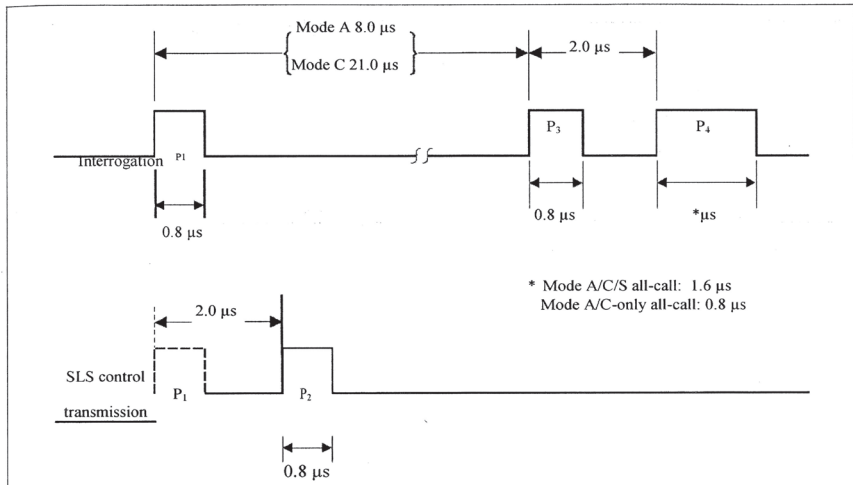
Figure 4-2 Intermode interrogation pulse sequence.
