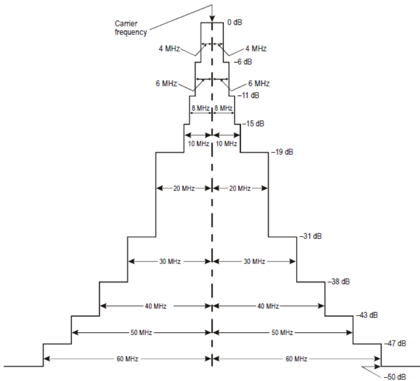
Figure 4-1 Required Spectrum limits for interrogator transmitter
