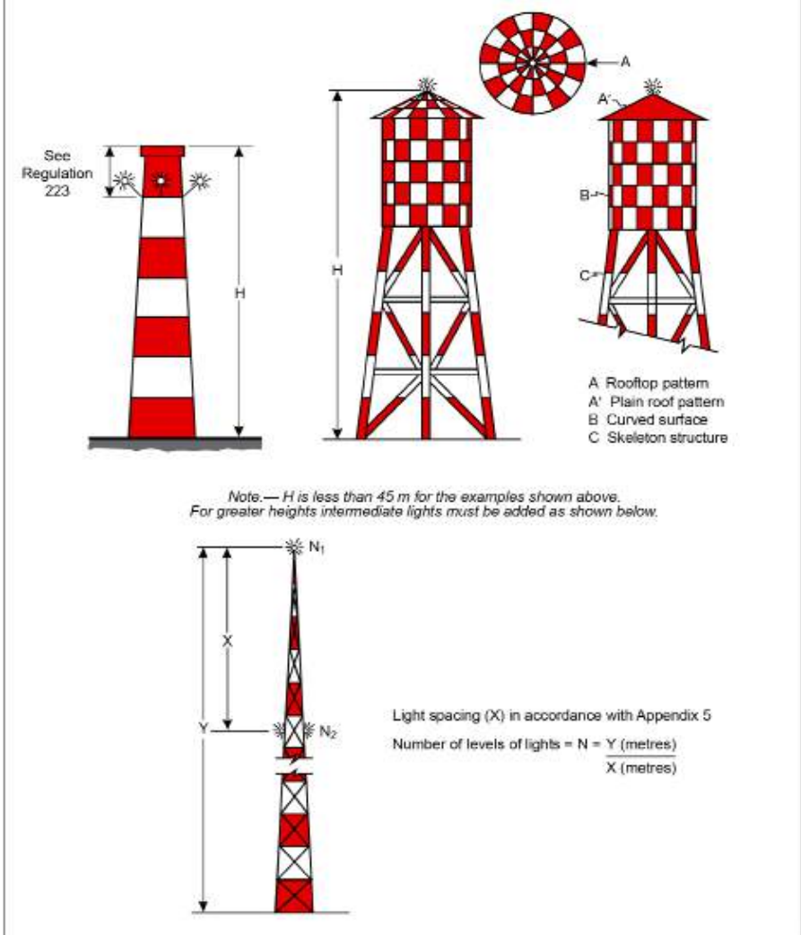
Figure 38: Marking and lighting of tall structures
