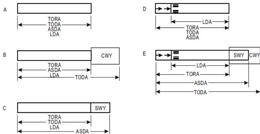
Figure S8-1. Illustration of declared distances
