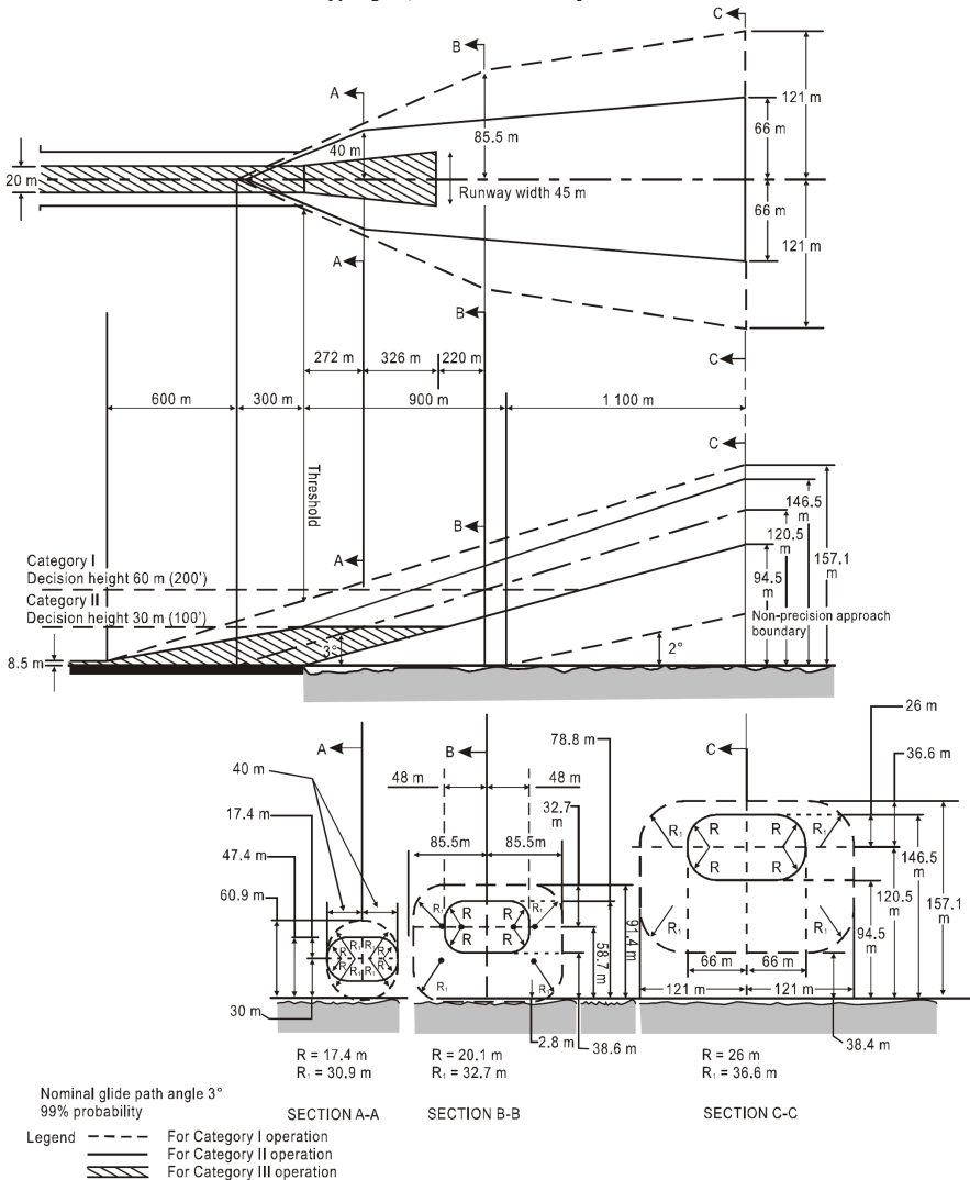
Figure S8-6. Flight path envelopes to be used for lighting design for category I, II and III operations
