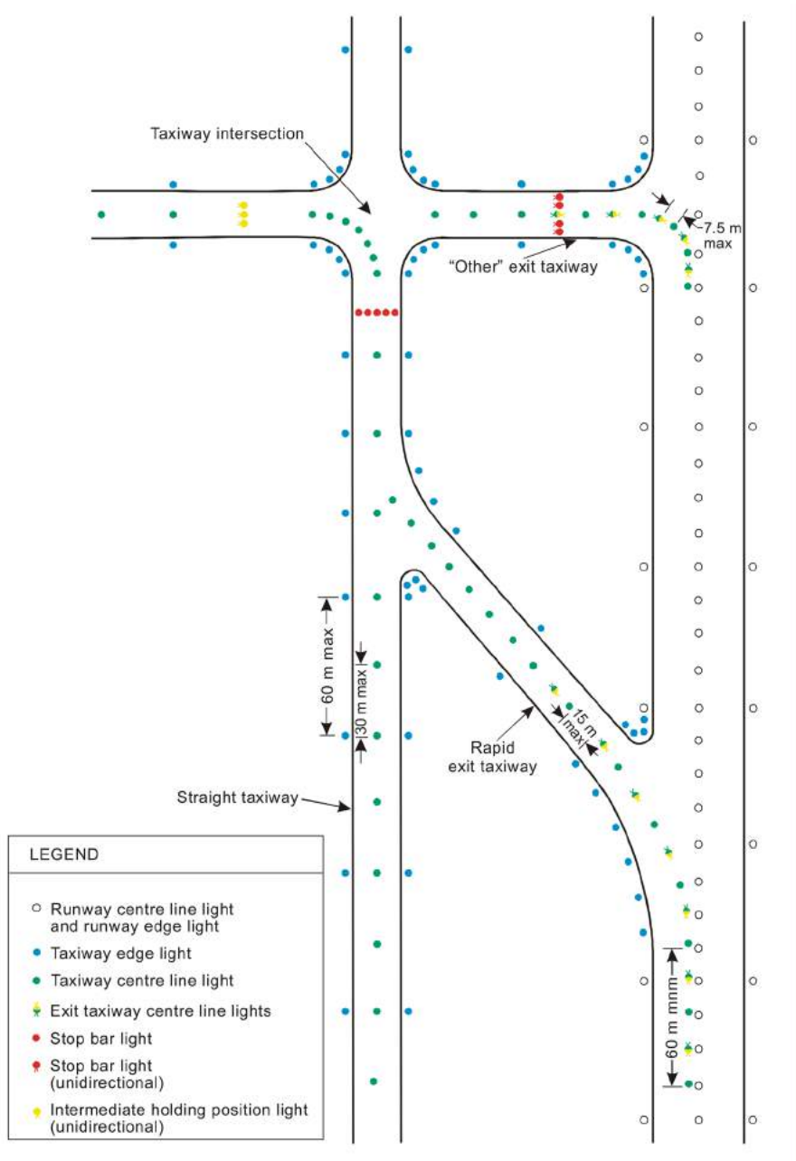
Figure 29: Taxiway lighting
