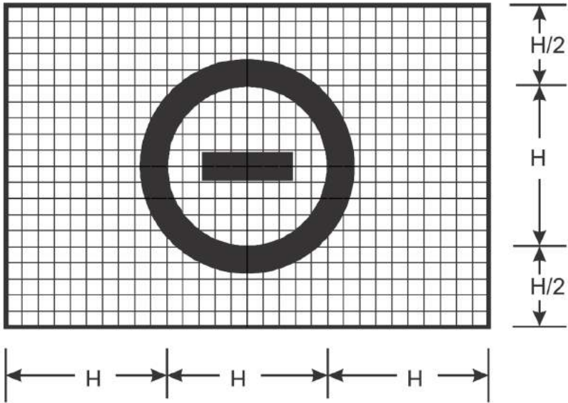
Figure S6-3. Sign dimensions
