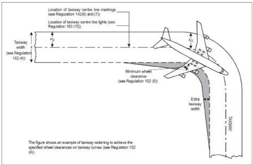
Figure 2. Taxiway curve
