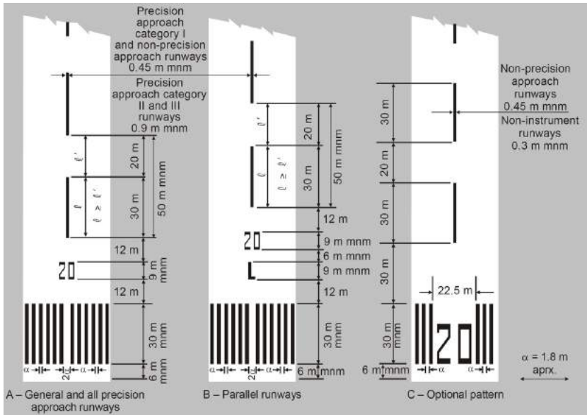
Figure 7 Runway designation, center line and threshold markings
