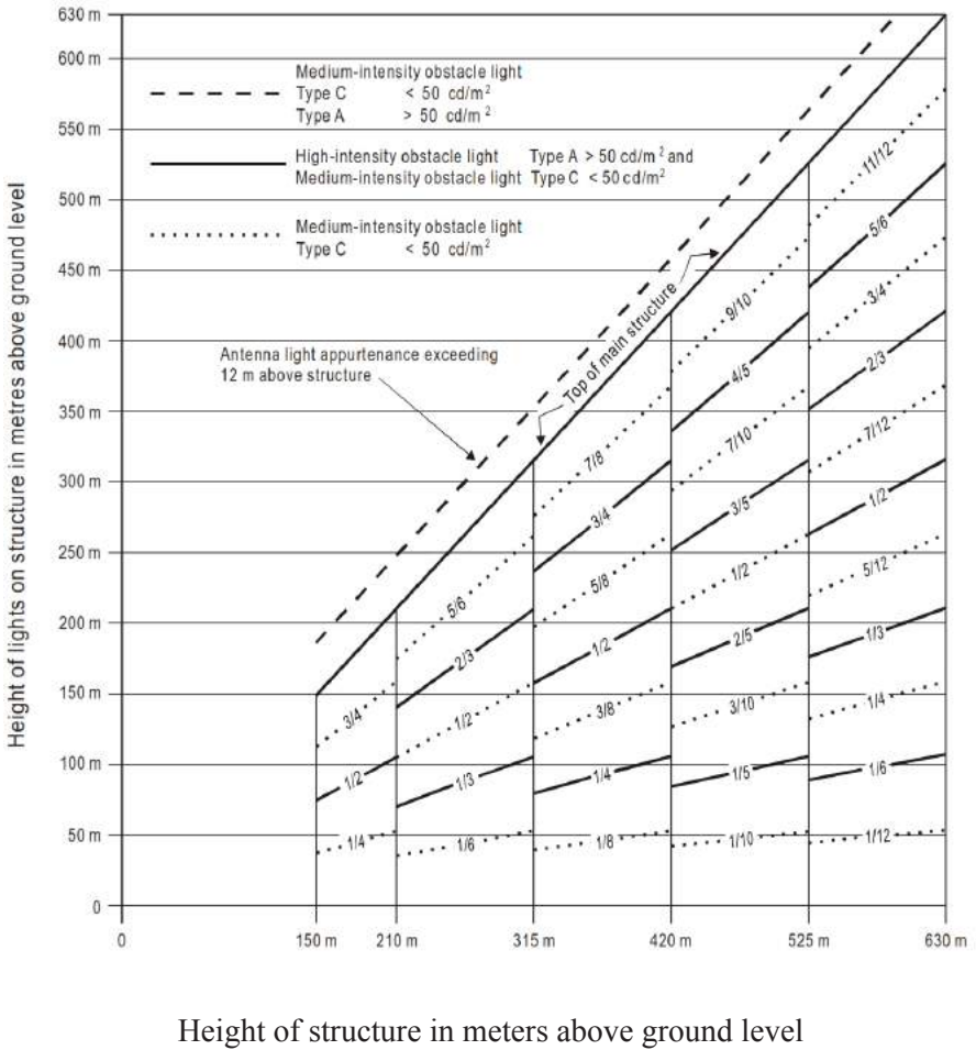
Figure S7-8. High-/medium-intensity dual obstacle lighting system, Type A/Type C
