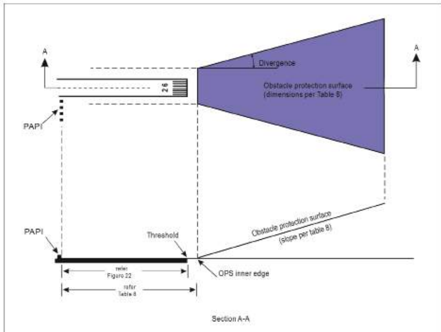
Figure 24 OPS for visual approach slope indicator systems
