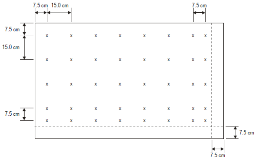
Figure S6-1. Grid points for calculating average luminance of a sign
