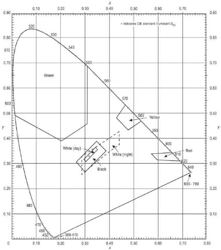
Figure S3-4. Colours of luminescent or transilluminated (internally illuminated) signs and panels
