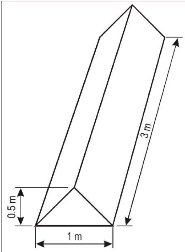
Figure 36 Boundary Markers
