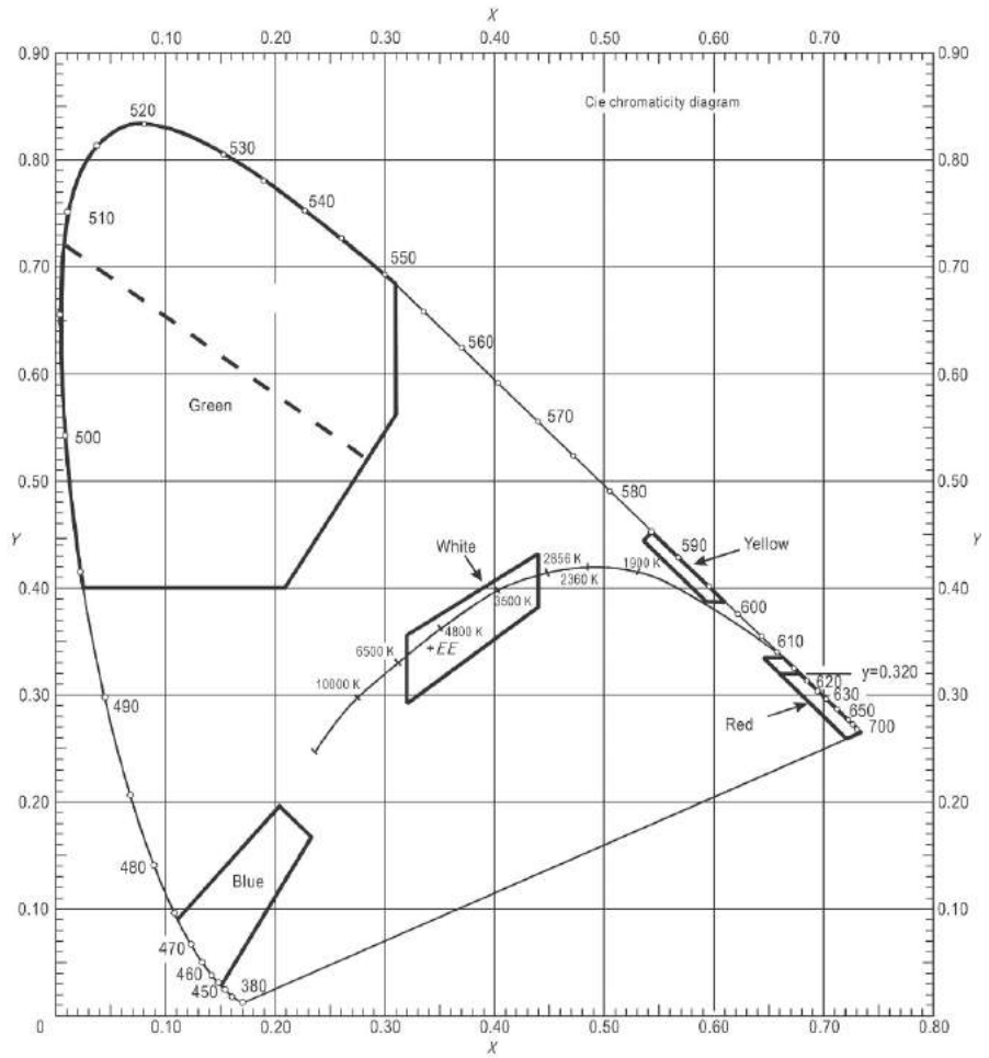
Figure S3-1b. Colours for aeronautical ground lights (solid state lighting)
