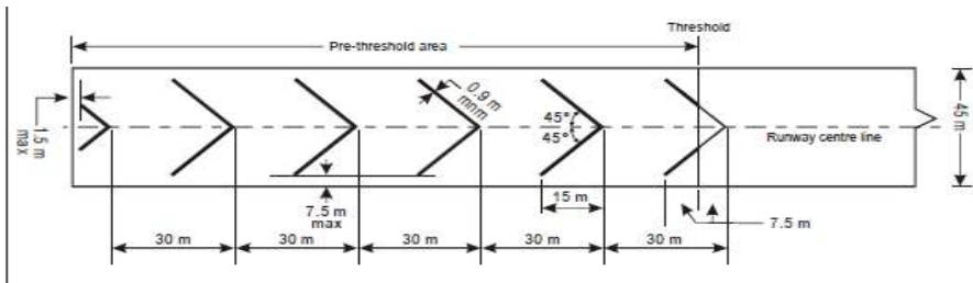
Figure 40. Pre-threshold marking
