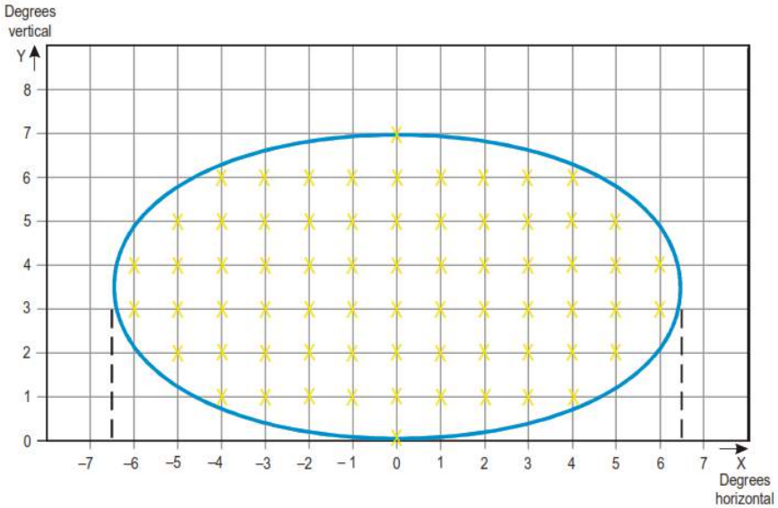
Figure S4-10. Isocandela diagram for runway edge light where width of runway is 60m (white light)
