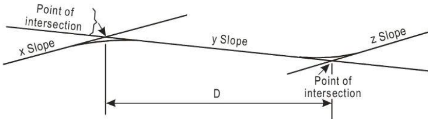
Figure S8-2. Profile on centre line of runway
