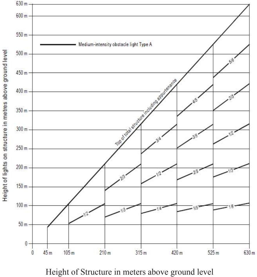
Figure S7-1. Medium-intensity flashing-white obstacle lighting system, Type A
