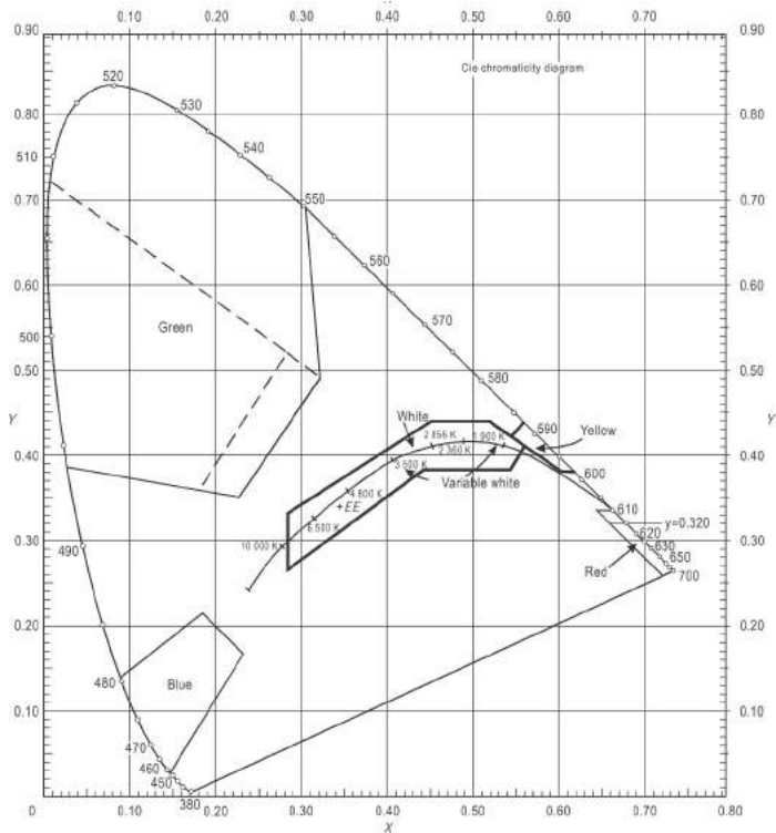
Figure S3-1a. Colours for aeronautical ground lights (filament-type lamps)
