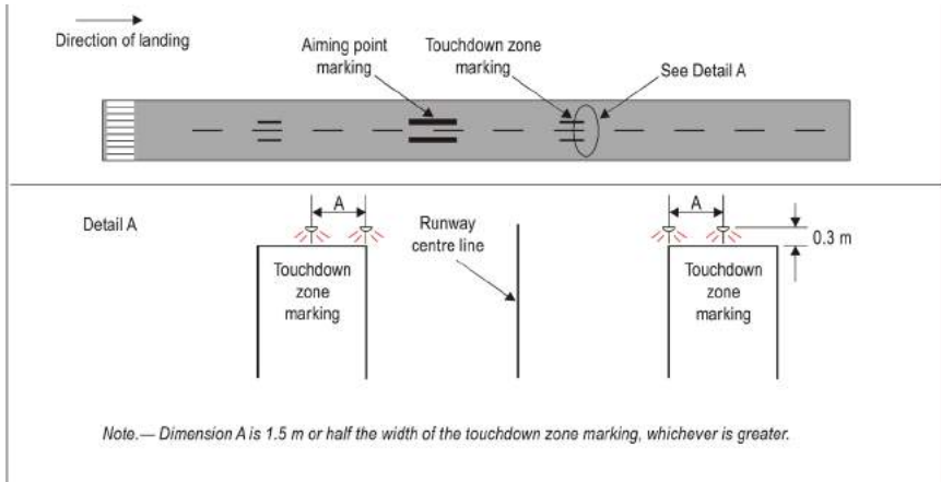
Figure 27: Simple touchdown zone lighting
